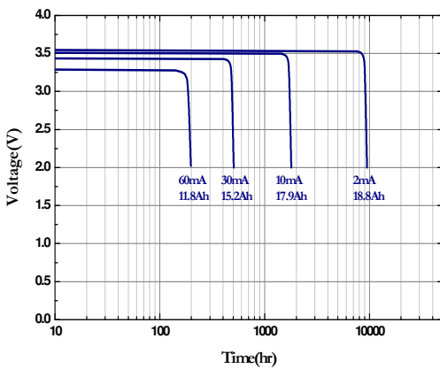
Continuous Discharge at 20°C
