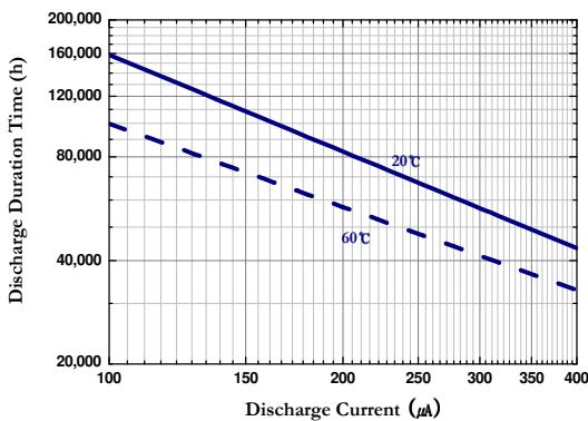
Discharge Current vs. Duration Time
