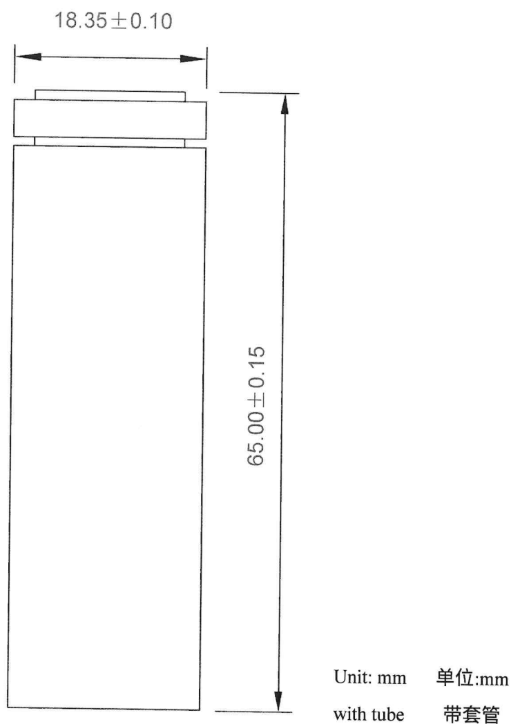
Fig. 1. Outline Dimensions of ICR18650/26V
