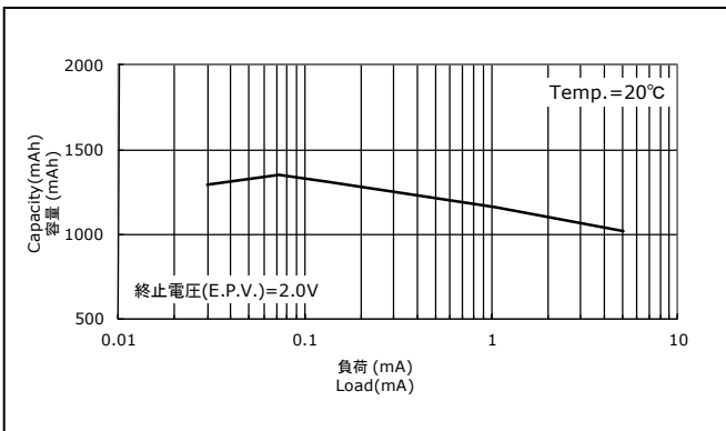
Discharge Load vs. Cell Capacity of CR2/3 6·L
